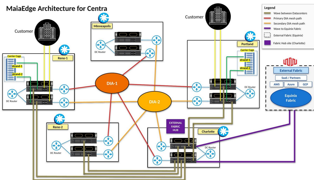
Figure 1. MaiaEdge federated architecture across CENTRA's five primary sites. Charlotte hosts the External Fabric Hub; waves connect Portland, Reno-1, and Reno-2 to Charlotte; Minneapolis reaches the fabric via DIA mesh.
